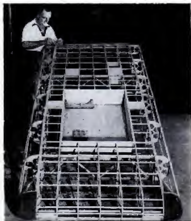
Boat is quickly detached from plane. Shaped like an airplane wing, it provides added lifting force in flight
